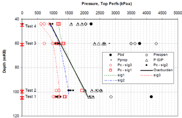
Figure 4. Mini-frac results for the 05-22 well
