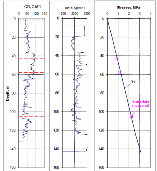
Figure 5. Mini-frac results for the 09-21 well
