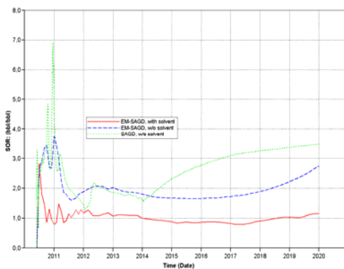
Figure 15. Comparison of steam-oil ratio (SOR) for EM-SAGD and SAGD process
