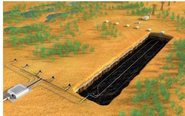
Figure 13. Artist impression of EM loop with on the left hand the well pad and the right hand top the induction loops power feed
