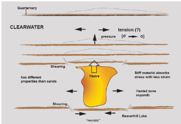
Figure 6. Main geomechanical mechanisms
