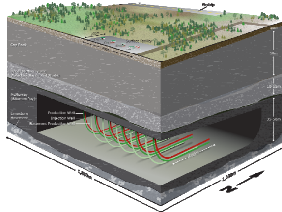
Figure 3. Artist view of Clearwater Phase I
