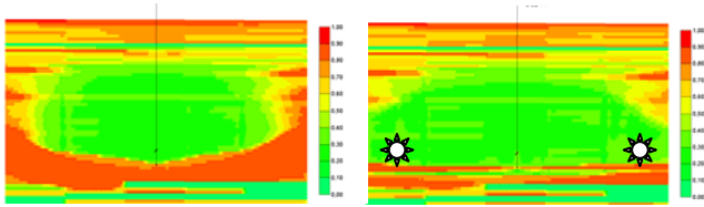
Figure 14 Oil saturation after 10 years: SAGD (left) and EM-SAGD (right). White symbols indicate the positions of the inductors.
