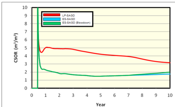
Figure 11. Calculated SLP-SAGD CSOR
