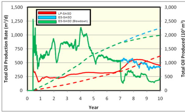
Figure 10. Predicted oil production rate
