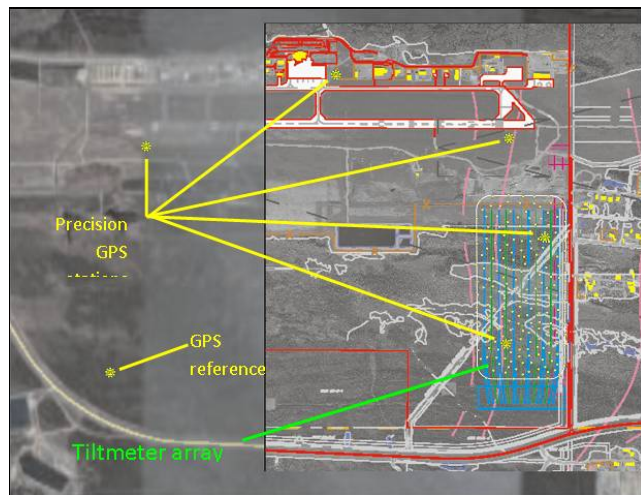
Figure 7. Area for diagnostic heave monitoring
